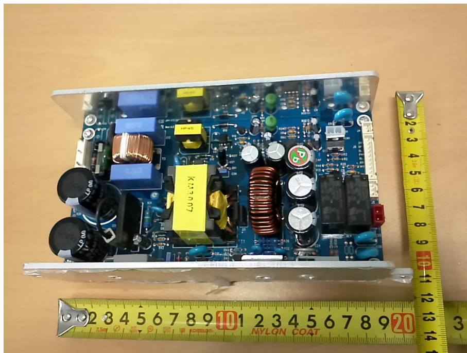
SMPS incorporating heat-sink
