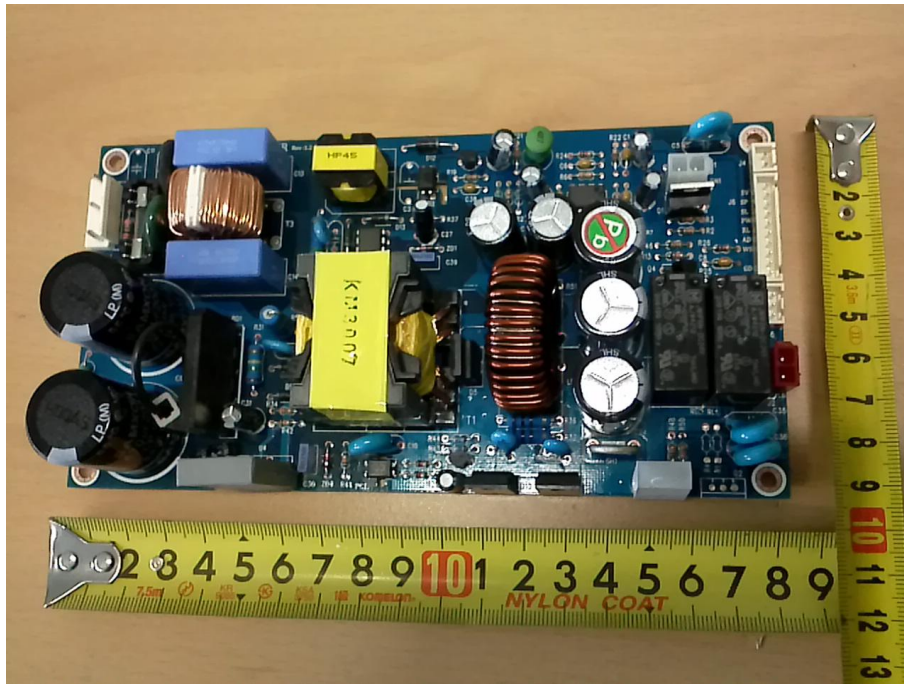
SMPS (Component side)
